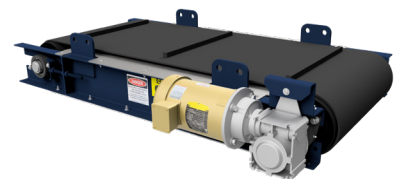
Overhead Self-Cleaning Permanent Magnet
